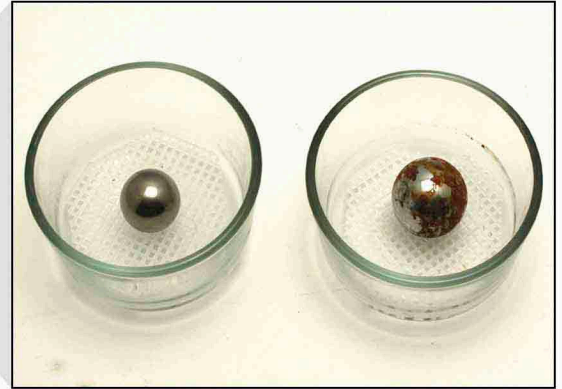
Good and Bad Material Tested in Salt Spray
